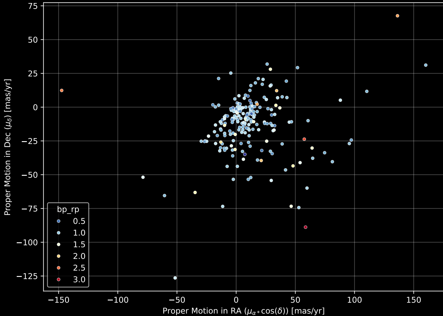
APOGEE DR17 Field: [174-51_MGA] Proper Motion Diagram (n= 214)
