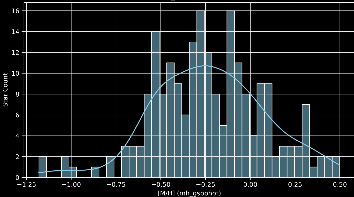
APOGEE DR17 Field: [174-51_MGA [M/H] (mh_gspphot) (n= 209)
