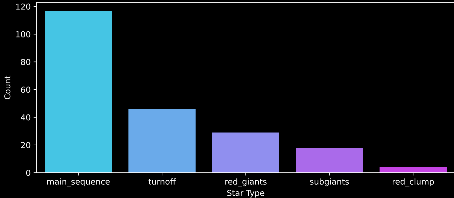
APOGEE DR17 Field: [174-51_MGA] Count plot of Star Type
