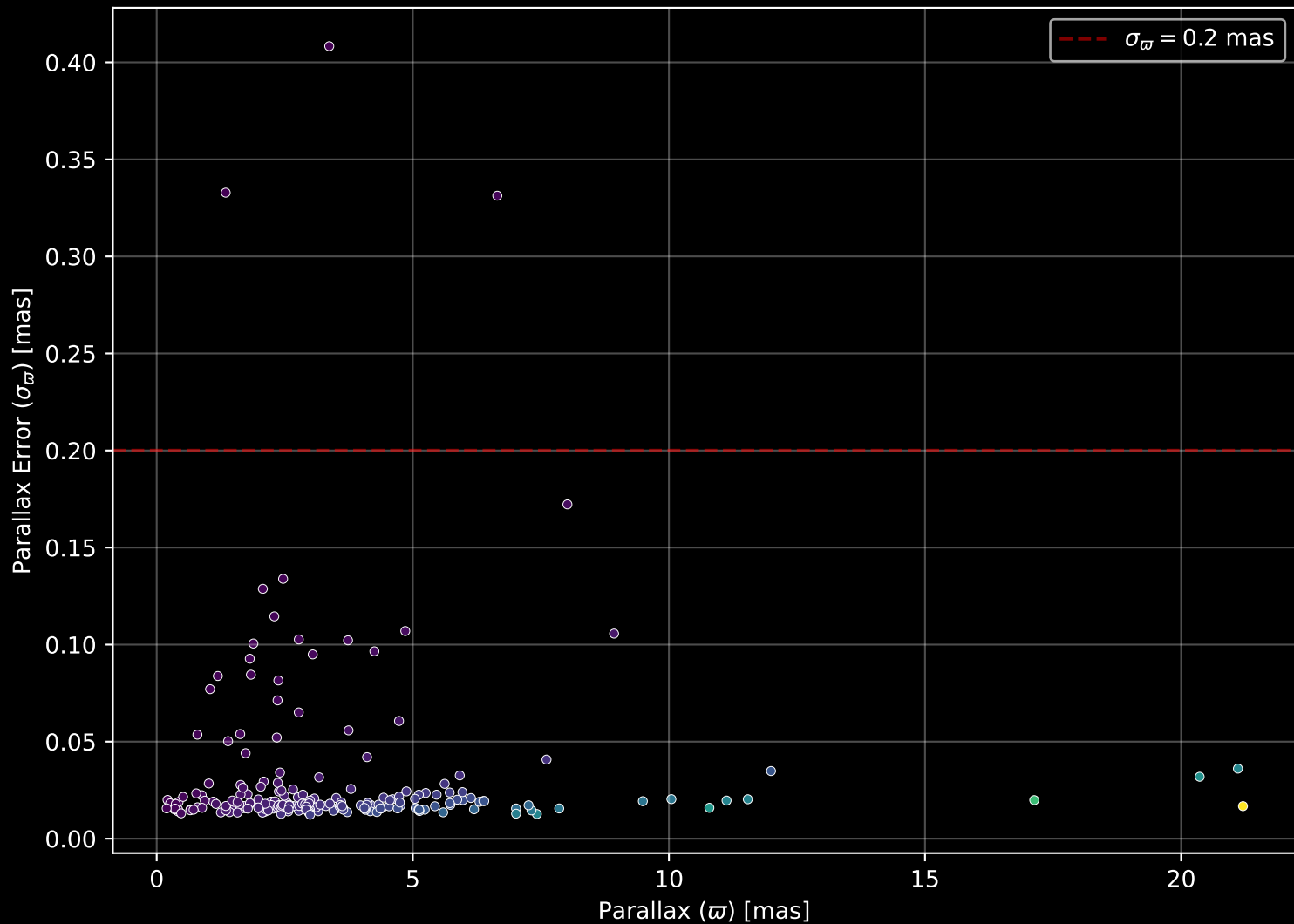
APOGEE DR17 Field: [174-51_MGA] Parallax Quality (n= 214)
