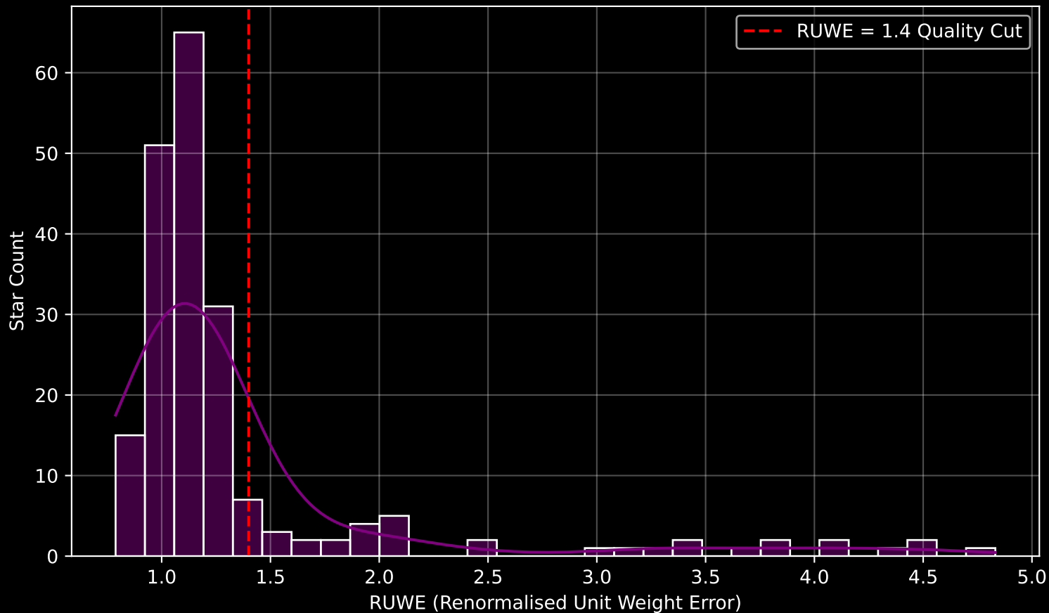
GAPOGEE DR17 Field [174-51_MGA] RUWE Distribution (n= 201)
