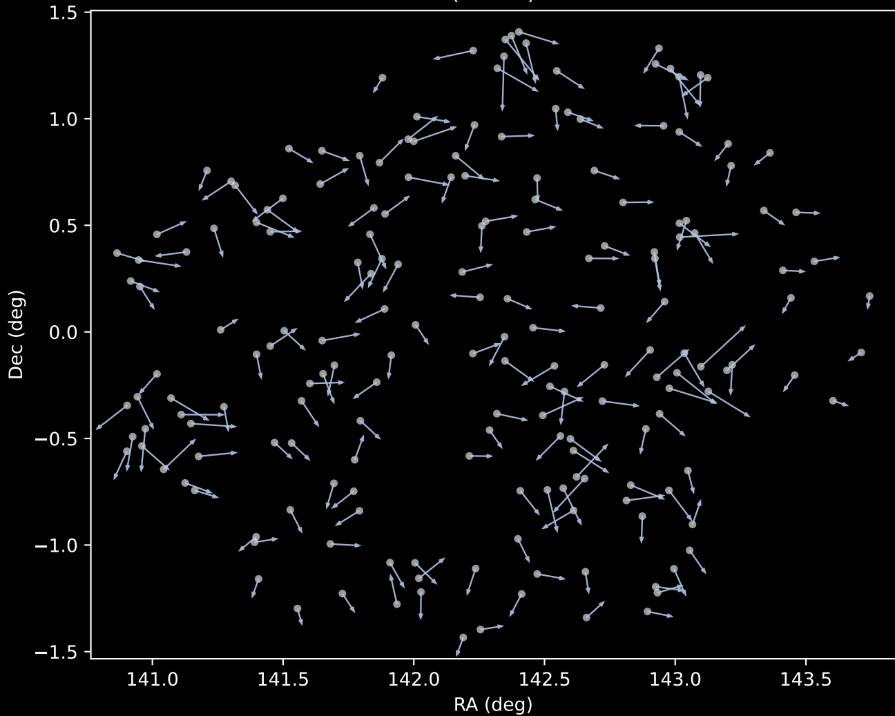
APOGEE DR17 Cluster 1 Proper Motion Vectors (n=186)
