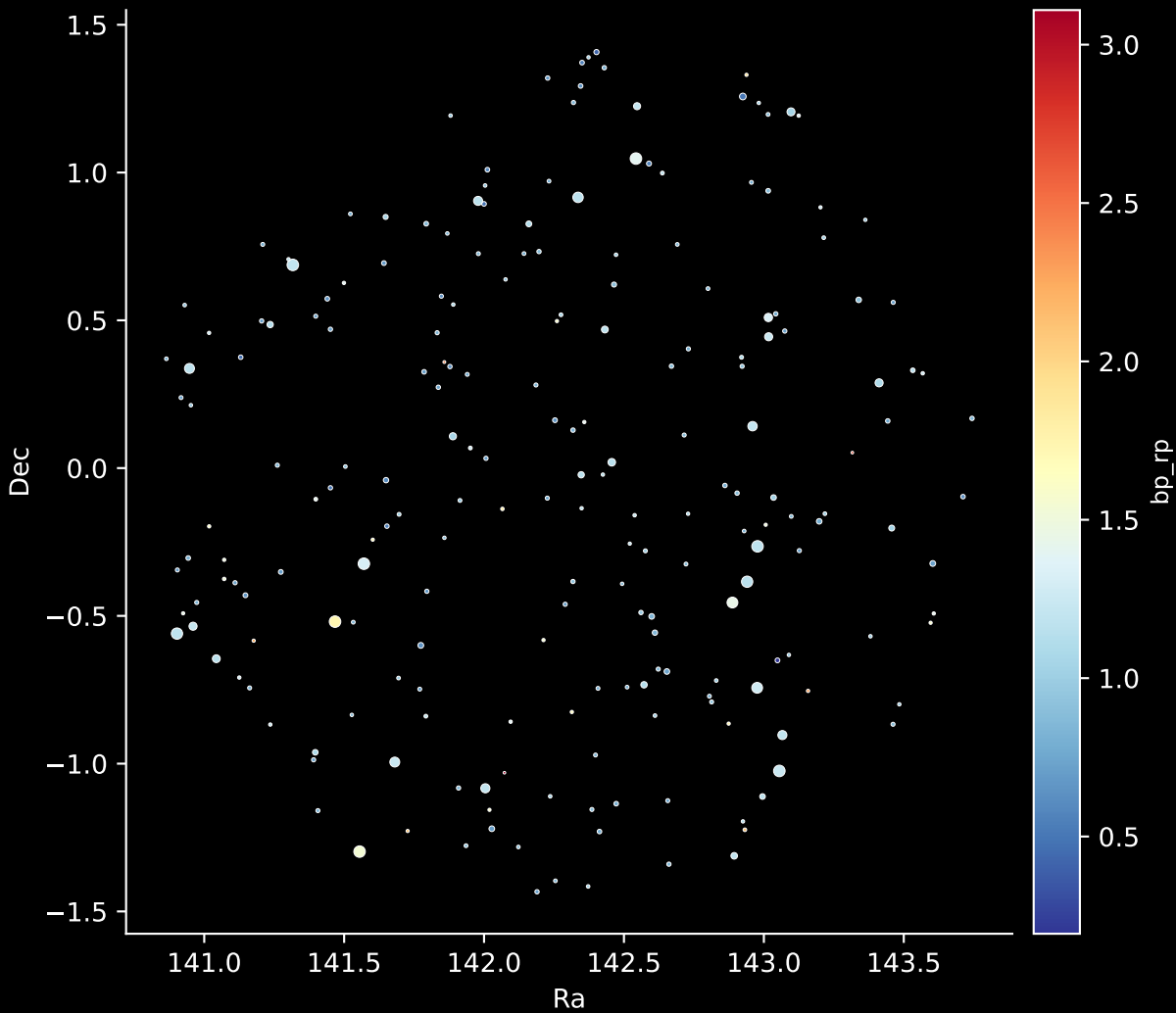
APOGEE DR17 Field: [174-51_MGA] Stars: 214
