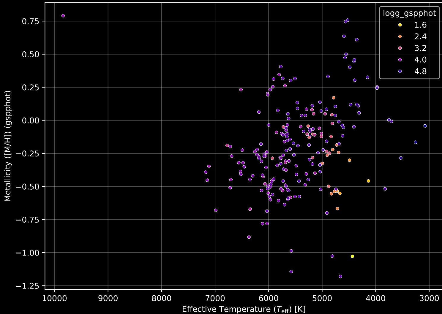
APOGEE DR17 Field: [174-51_MGA] Stellar Population Parameters (n= 214)
